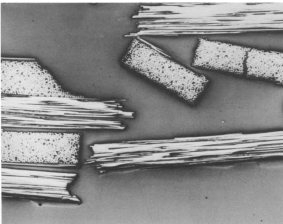
Figure 11 Bending tensile failure of a 5208 epoxy-T-300 carbon fibre composite. Delamination extends well beyond field of view.
