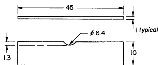
Figure 1 Microbeam sample geometry. All dimensions in mm.
