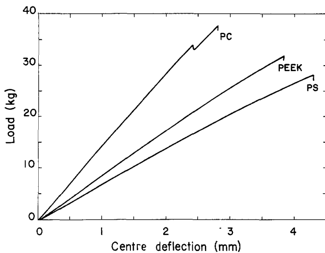
Figure 7 Typical load-deflection curves of composite microbeam samples in four-point bending.
