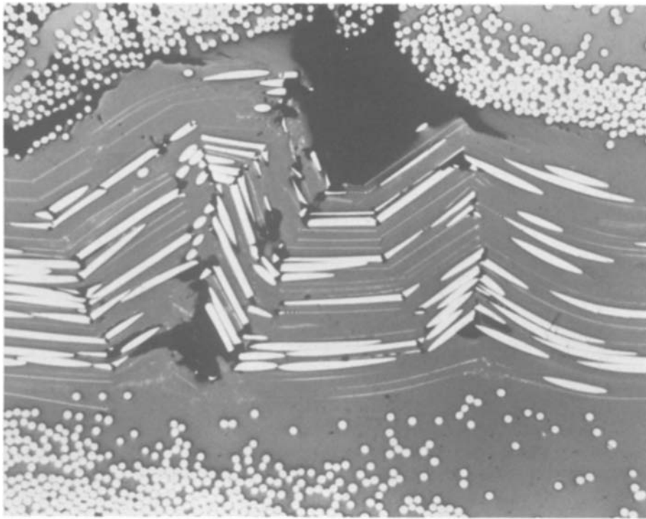
Figure 9 Microbuckling failure of the third ply in a PC-AS-4 composite. Constraint by neighboring plies allows several kinks to form.
