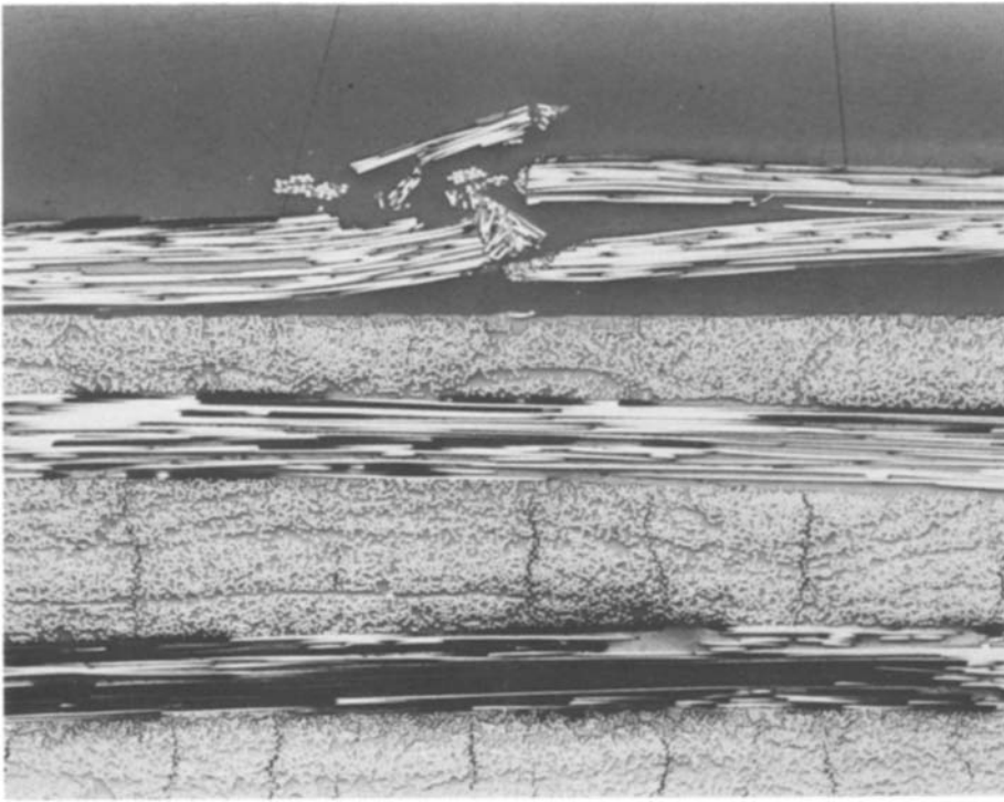
Figure 12 Bending compression failure in a PPS-C-6000 composite that has been annealed to produce high matrix crystallinity. Notice transverse cracks which are present before bending the sample. Compare failure to Fig. 5.
